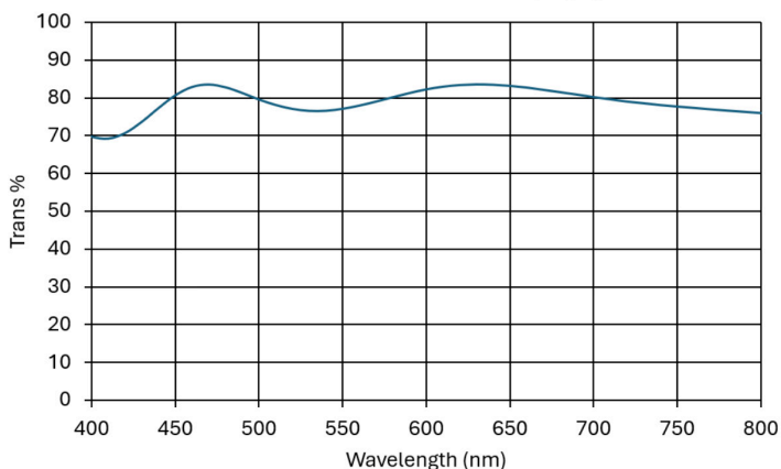
Transmission at 45° in visible (Fig 1)
