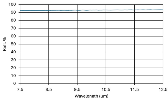
Reflection at 45° AOI in Far Infra-Red (Fig 2)
